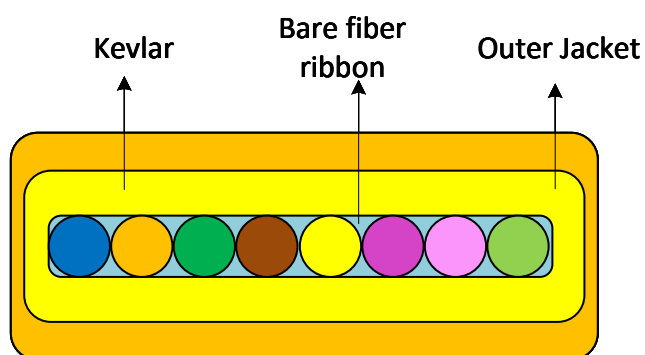
Cable Structure
