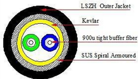
cable structure
